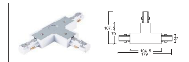
3線A T接頭-右 T-connector - R
