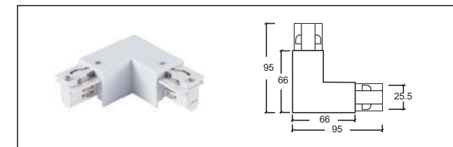
H-02 L 型接頭-右 L-connector - R
