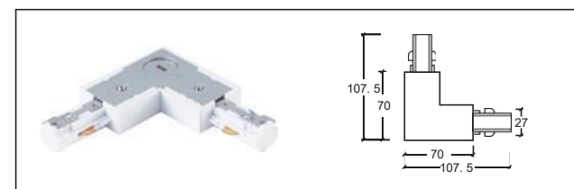
3線A L型接頭-左 L-connector - L
