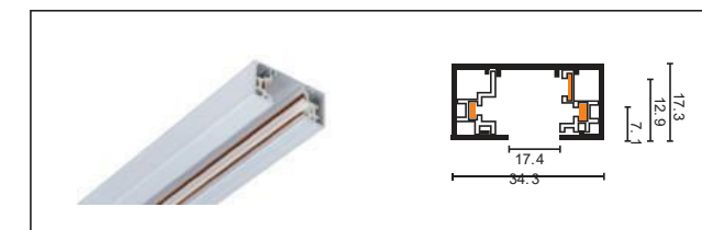
3線A型美規軌道條 Three Line ASA Track
