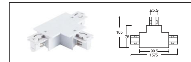
H-03 T接頭-右 T-connector - R
