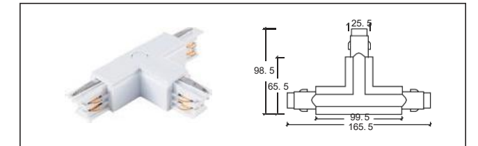
H-04 T接頭-右 T-connector - R
