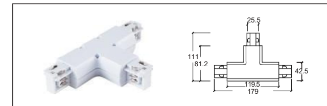
H-01 T接頭-右 T-connector - R
