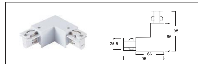
H-02 L 型接頭-左 L-connector - L
