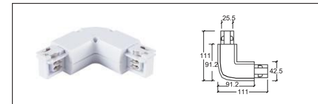
H-01 L 型接頭-右 L-connector - R
