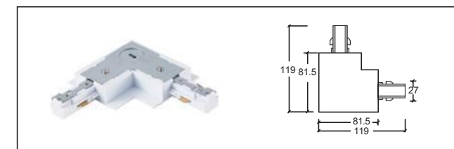
3線A 嵌入式L型接頭-右 L-connector - R
