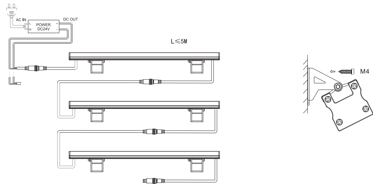
Each set of line strips has a maximum length of 5 meters Please ensure that it is carried out in case of power failure during installation and maintenance.
